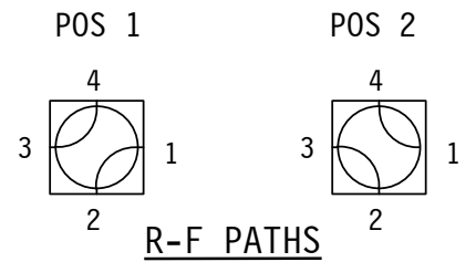
STD. ELECT. CKT. Shown in Pos. 1 ONE FORM C
