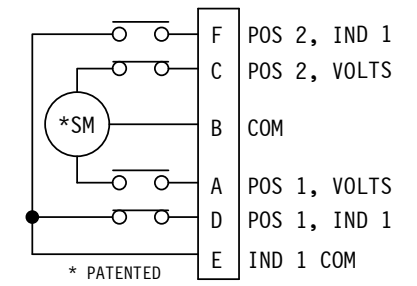
STD. ELECT. CKT. Shown in Pos. 1 ONE FORM C
