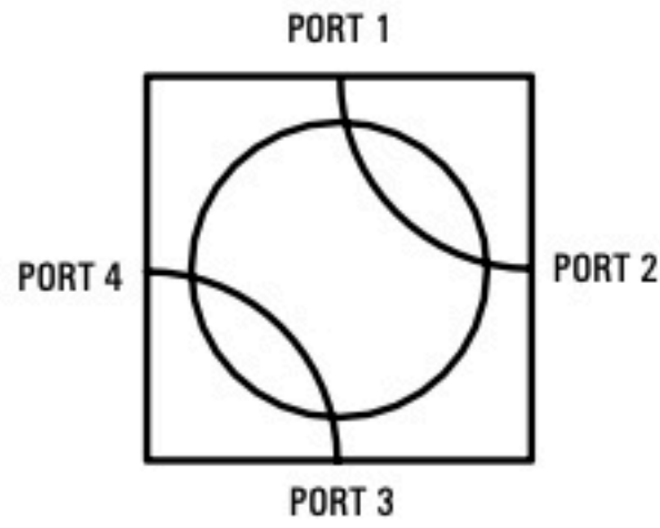
POSITION 1 OF THE RF PORTS
