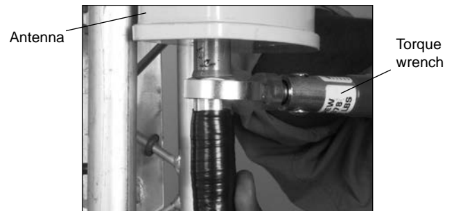
Tighten connection
